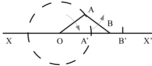
Figure 2: Simple Harmonic Motion as Birotation
