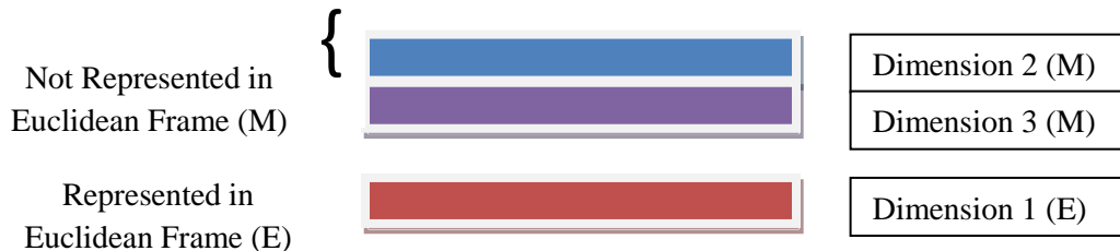
Fig 1. “Electric” and “Magnetic” Dimensions of Motion
