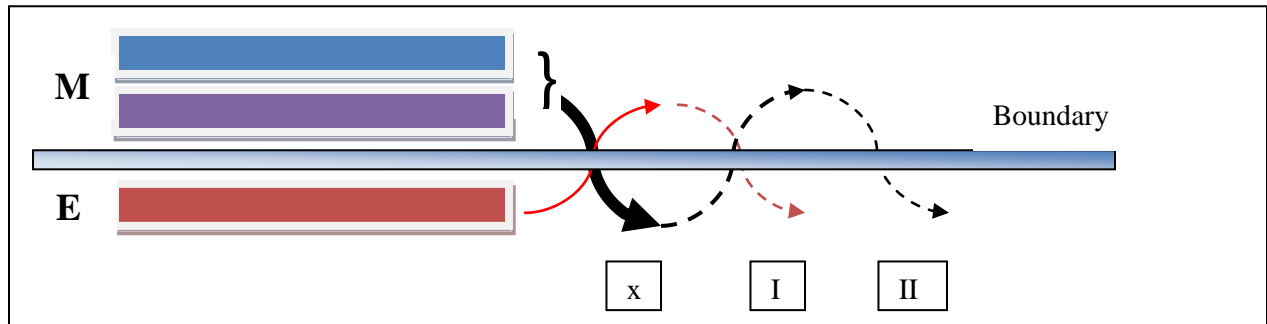
Fig. 3 Muon Magnetic Moment Increments
