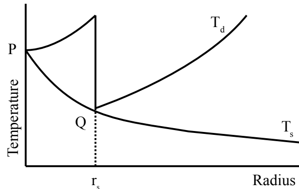
Figure 3: Onset of Secondary Burning
