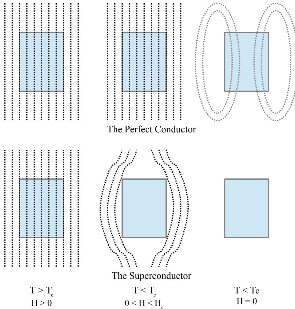
Figure 1: The Meissner Effect
